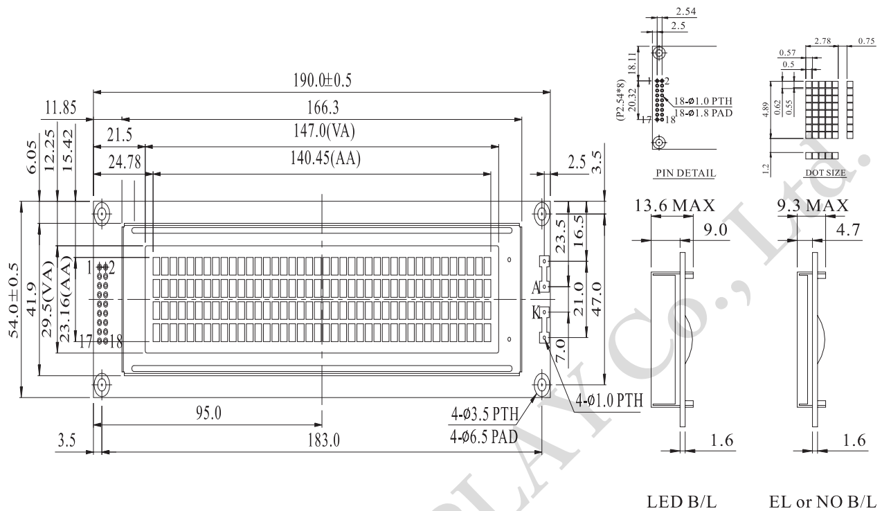
Dimension drawing
